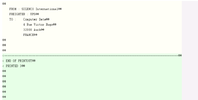
Figure 12 File footer
