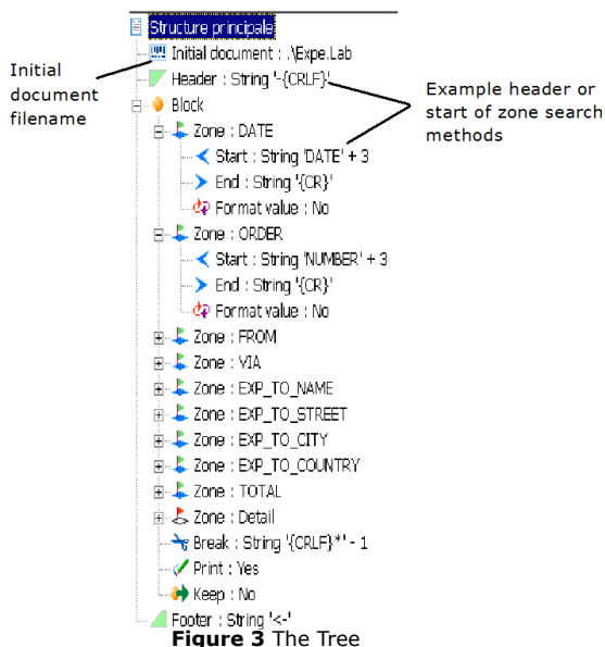
Figure 3 The Tree
